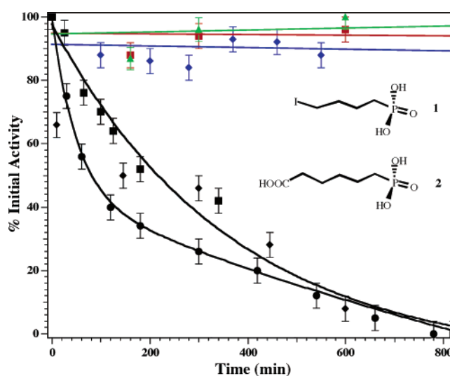
FIGURE 5: Reaction of 1 with WT EcMetAP-I (black squares 30 mM, black diamonds 10 mM), WT PfMetAP-II (green triangles, 10 mM), C59A EcMetAP-I (red squares, 10 mM), and C70A EcMetAP-I (black circles, 10 mM). Reaction of a 30 mM solution of 2 with WT EcMetAP-I (blue diamonds). Reaction conditions: 1 \mu M Co(II)-loaded MetAP in 50 mM HEPES buffer, pH 7.5, 150 mM KCl under anaerobic conditions.
