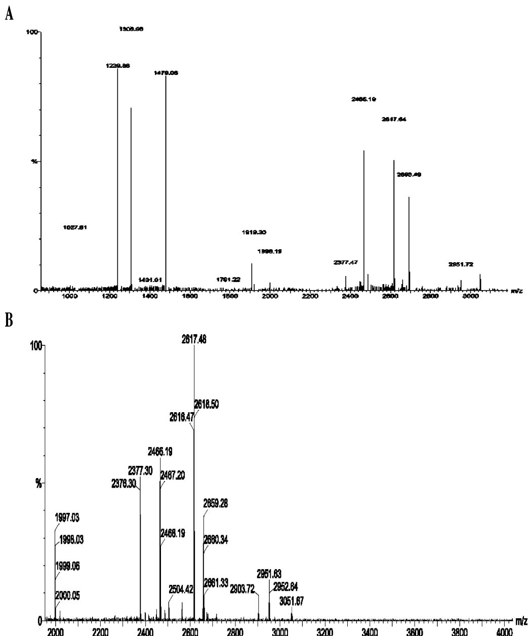
FIGURE 4: MALDI-TOF MS of tryptic digested samples of (A) Co(II)-loaded WT EcMetAP-I and (B) Co(II)-loaded WT EcMetAP-I + DTNB.
