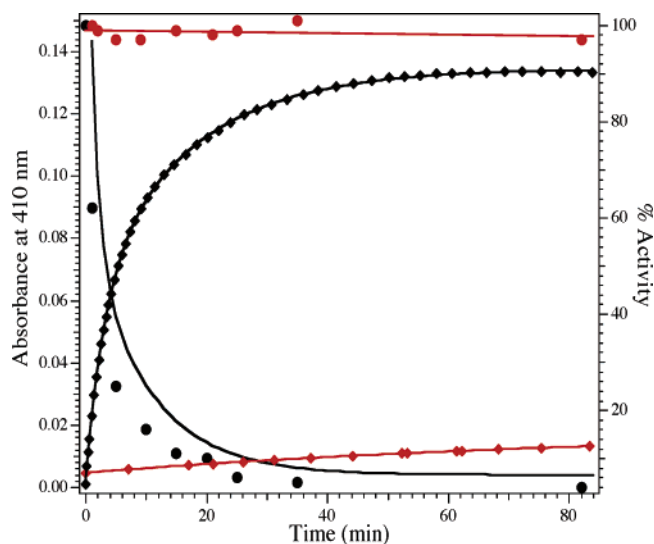
FIGURE 3: Activity as a function of time for EcMetAP-I (black circles) and PfMetAP-II (red circles) after reaction with 200 \mu\text{M} DTNB. DTNB absorbance after reaction with EcMetAP-I (black diamonds) and PfMetAP-II (red diamonds). Reaction conditions: 1 \mu\text{M} Co(II)-loaded MetAP in 50 mM HEPES buffer, pH 7.5, 150 mM KCl under anaerobic conditions.
